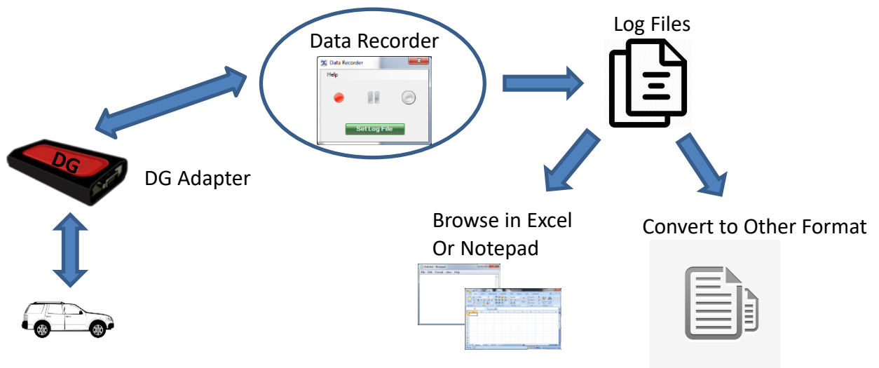
Figure 2 - Standalone Mode
