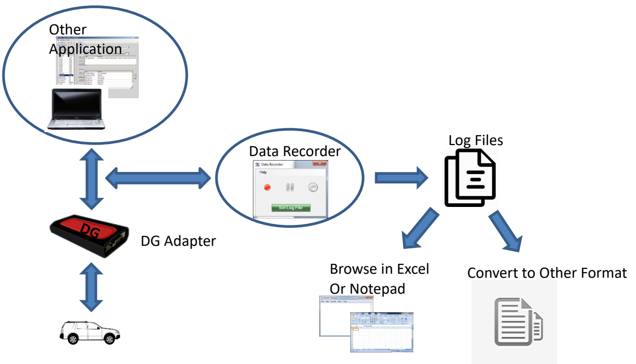
Figure 3 - Dependency Mode
